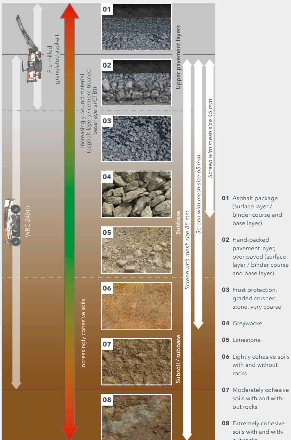
Range of Applications Rock Crusher WRC 240 (i)
