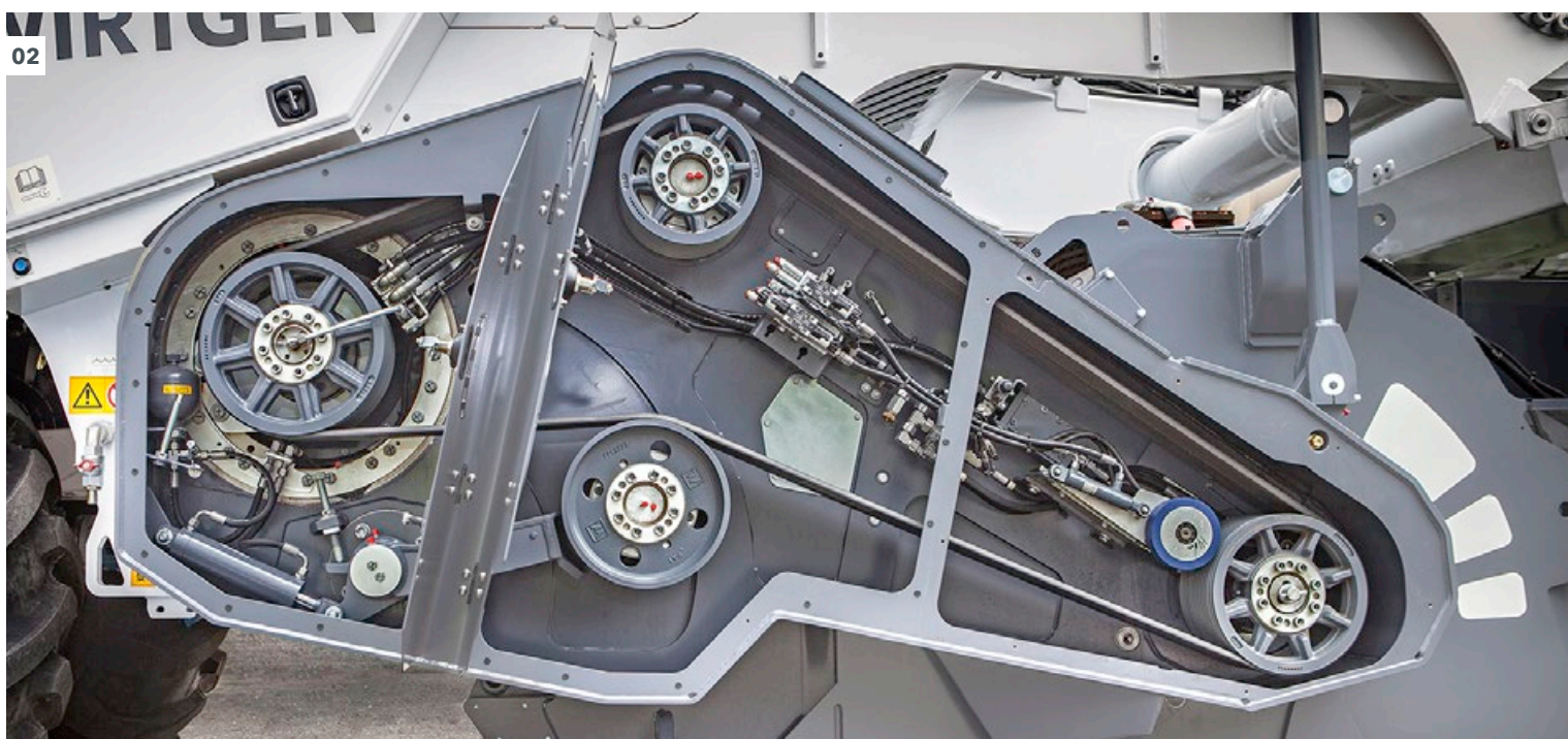
02 Belt drive for the crushing and mixing rotor.
