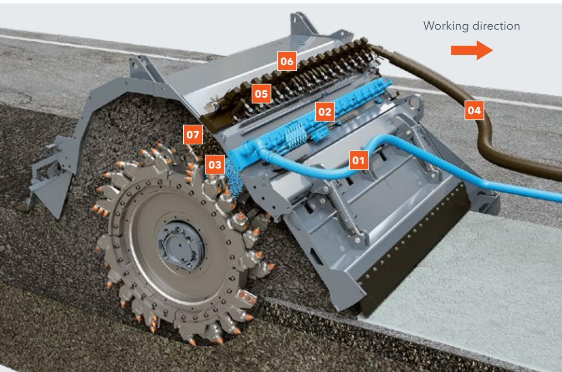
01 The filling connector for foamed bitumen is easily accessible.
