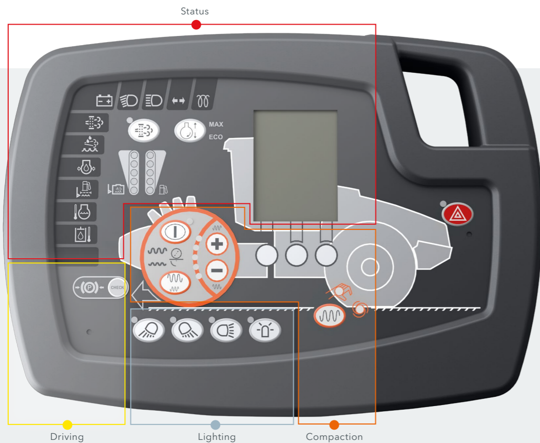
The dashboard behind the steering wheel contains status and parameter displays as well as infrequently used buttons. All displays and switches are grouped into functional units with colour markings. This makes operation easier, since the same applies here as it does to all other HAMM rollers: Same colour - same functional group.
